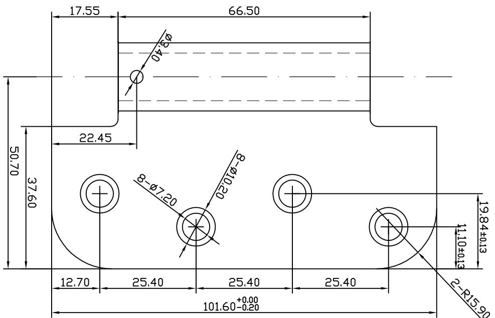
IMPORT SPRING 4"X4"X2.7mmSQ-5/8" RIGHT
